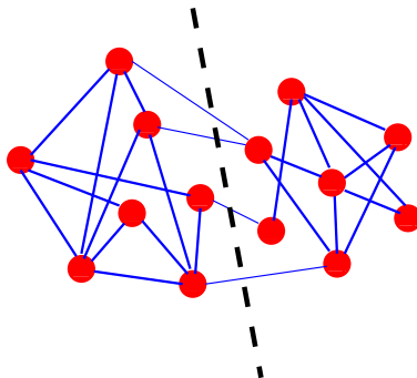
Figure 5: Graph partitioning. The cut shows the partition in two groups of equal size.
