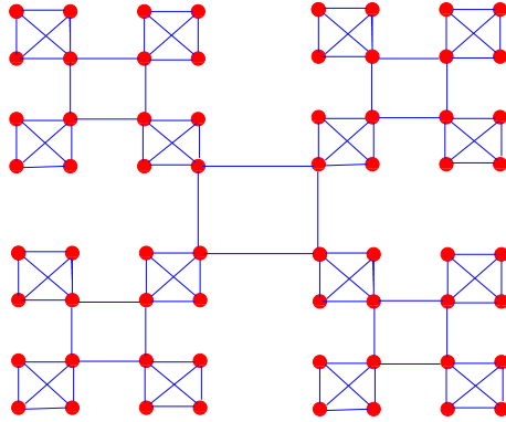
Figure 2: Schematic example of a hierarchical graph. Sixteen modules with four vertices each are clearly organized in groups of four.
