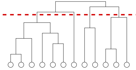
Figure 3: A dendrogram, or hierarchical tree. Horizontal cuts correspond to partitions of the graph in communities. Reprinted figure with permission from Newman MEJ, Girvan M, Physical Review E 69, 026113, 2004. Copyright 2004 by the American Physical Society.
