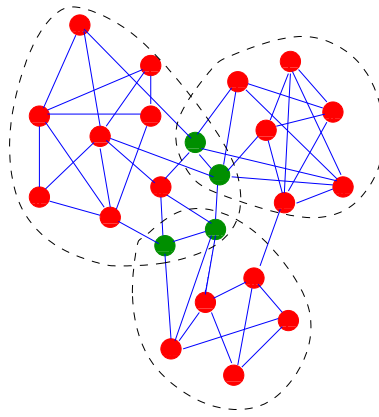
Figure 4: Overlapping communities. In the partition highlighted by the dashed contours, the green vertices are shared between more groups.
