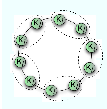
Figure 7: Resolution limit of modularity optimization. The natural community structure of the graph, represented by the individual cliques (circles), is not recognized by optimizing modularity, if the cliques are smaller than a scale depending on the size of the graph. Reprinted figure with permission from Fortunato S, Barthélemy M, Proceedings of the National Academy of Science of the USA, 104, 36 (2007). Copyright 2007 from the National Academy of Science of the USA.
