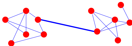
Figure 6: Edge betweenness is highest for edges connecting communities. In the figure, the thick edge in the middle has a much higher betweenness than all other edges, because all shortest paths connecting vertices of the two communities run through it.
