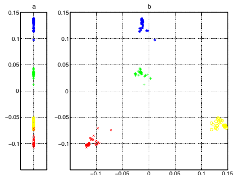
Figure 8: Spectral algorithm by Donetti and Muñoz. Vertex i is represented by the values of the i th components of Laplacian eigenvectors. In this example, the graph has an ad-hoc division in four communities, indicated by the colours. The communities are better separated in two dimensions (b) than in one (a). Reprinted figure with permission from Donetti L, Muñoz MA, Journal of Statistical Mechanics: Theory and Experiment, P10012 (2004). Copyright 2004 by the Institute of Physics.
