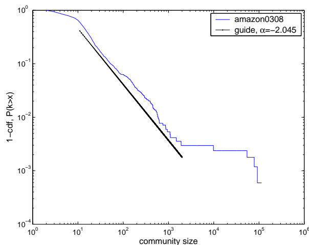
Figure 13: Cumulative distribution of community sizes for the Amazon purchasing network. The partition is derived by greedy modularity optimization. Reprinted figure with permission from Clauset A, Newman MEJ and Moore C, Physical Review E 70, 066111, 2004. Copyright 2004 by the American Physical Society.
