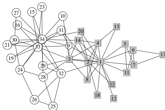
Figure 12: Zachary’s karate club network, an example of graph with known community structure. Reprinted figure with permission from Newman MEJ, Girvan M, Physical Review E 69, 026113, 2004. Copyright 2004 by the American Physical Society.
