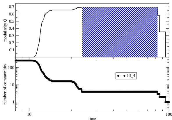
Figure 9: Number of clusters of synchronized Kuramoto oscillators as a function of time for a hierarchical graph. The two levels of community structure are revealed by the plateaus in the figure, which indicate the stability of those configurations. The top diagram shows the values of Newman-Girvan modularity Q for the corresponding partitions. The shadowed area highlights the partition with largest modularity. Reprinted figure with permission from Arenas A, Díaz-Guilera A, European Physical Journal ST 143, 19 (2007). Copyright 2007 by EDP Sciences.
