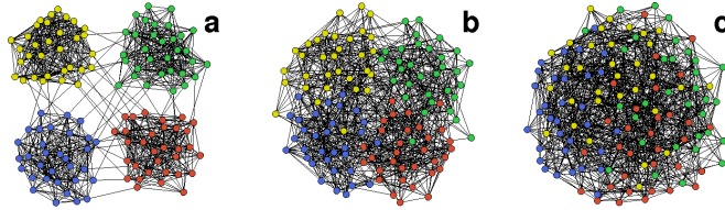
Figure 11: Benchmark of Girvan and Newman. The three pictures correspond to z_{in} = 15 (a), z_{in} = 11 (b) and z_{in} = 8 (c). In (c) the four groups are basically invisible. Reprinted figure with permission from Guimerà R, Amaral LAN, Nature 433, 895 (2005). Copyright 2005 by the Nature Publishing Group.
